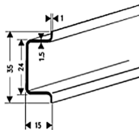
PR007 35 x 15 mm 2 Meter Steel Unslotted PR007-1M 1 Meter
