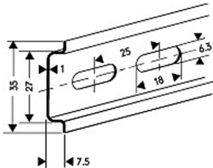
PR005 35 x 7.5 mm 2 Meter Steel Slotted PR005-1M 1 Meter
