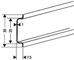
PR003 35 x 7.5 mm 2 Meter Steel Unslotted PR003-1M 1 Meter
